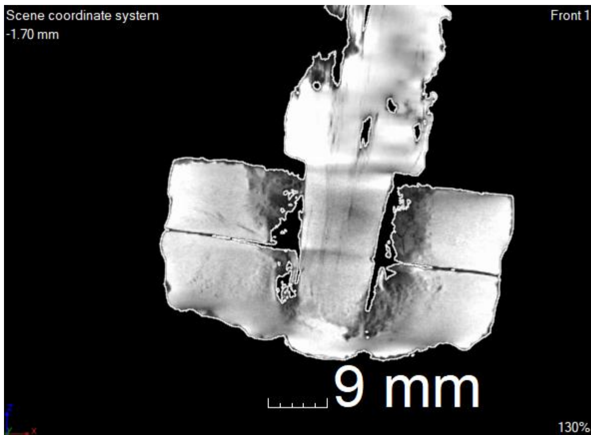
Figure S3. Varín sword. Frontal CT image of the pommel. Black structures represent corrosion pittings (elaborated by author, photo by J. Šurka).
